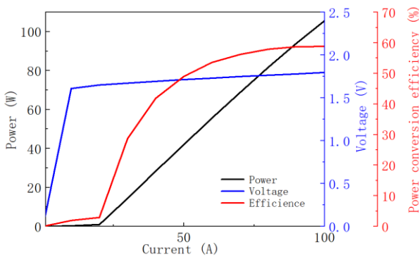
Power-Current-Voltage-Efficiency
